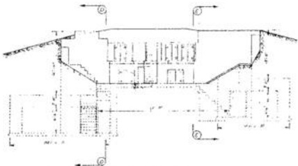
NORTH ELEVATION OF MAGAZINE #1 SCALE: 1/4" = 1'-0"
