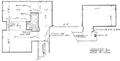
MAGAZINE #2 SCALE: 1/4" = 1'-0"
