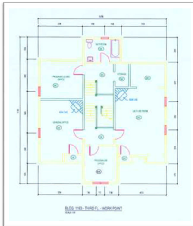
Figure 14. Second floor plan, WP 1163, Military Family Support Centre, Work Point Barracks, CFB Esquimalt (DND, 2011)
